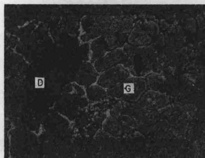
Figure 9.—Polished high-pressure orthorhombic \text{GdSb}_2 (500X).
